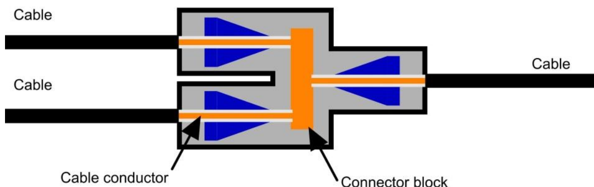
Figure 47 – Schematic Y-branch joint “Y” Joint Internal Schematic
