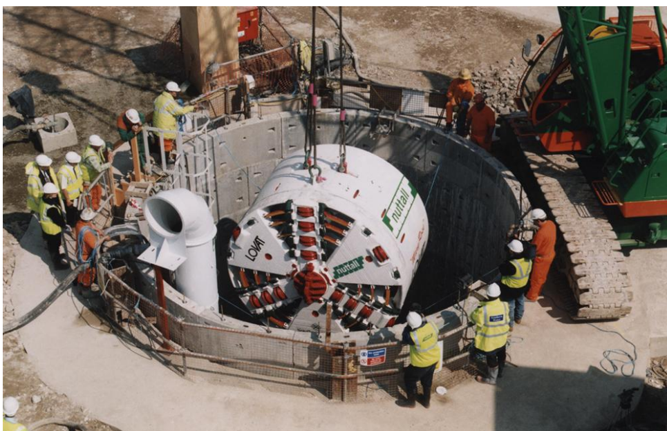
Figure 68 – Head-section of TBM being lowered into working shaft
