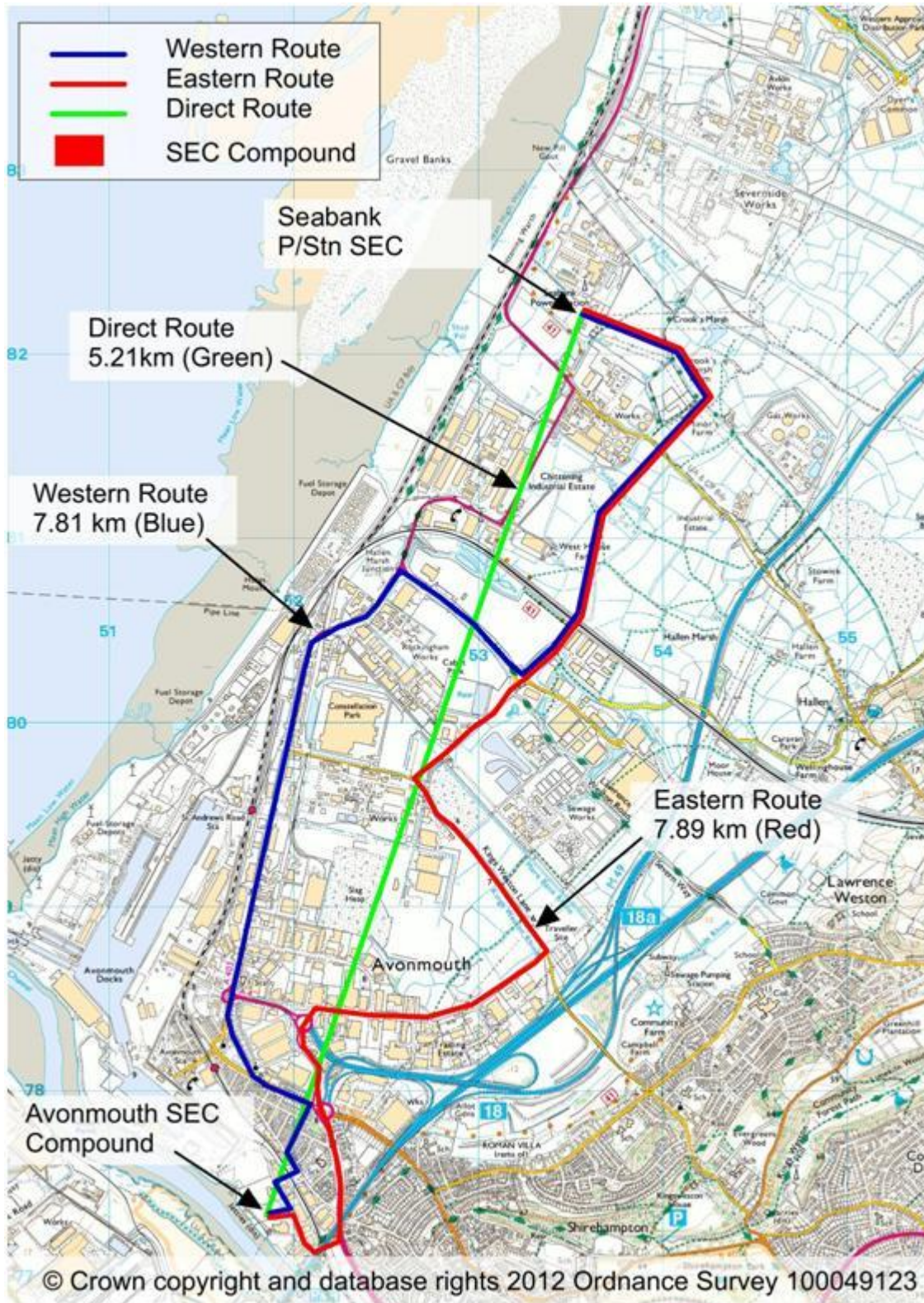
Figure 1 – Case study 1, UGC route Avonmouth
