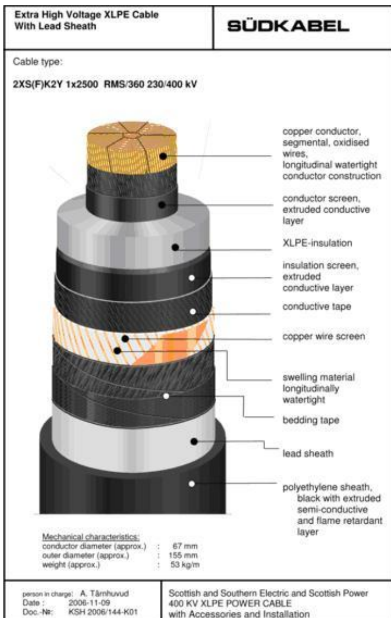
Figure 18 – Diagram of a 400kV transmission power cable
